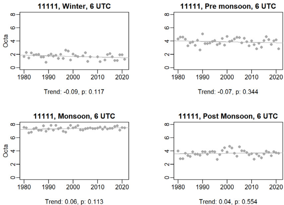
Figure 3.16: Trends in amount of cloud cover (oktas/decade) at Dhaka (11111)
